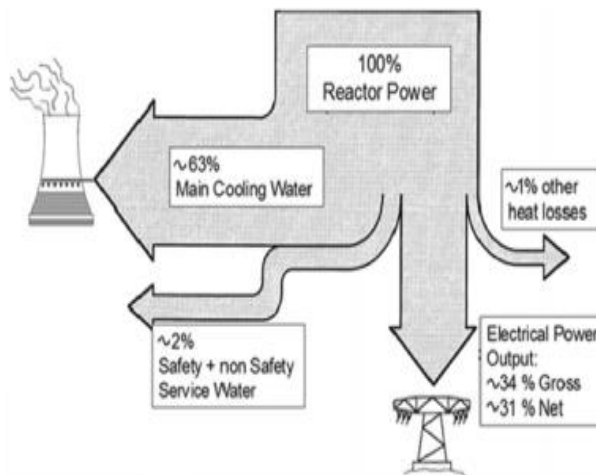
Figure 6-3: Energy conversion and heat dissipation during operation at full load Source: (IAEA, 2012) (No. NP-T-2.6)
