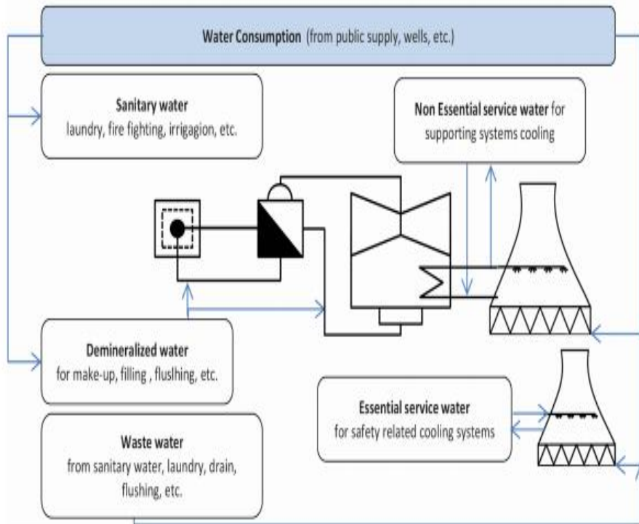
Figure 6-2: Water Streams in an NPP regarding consumption and withdrawal for closed cooling system
