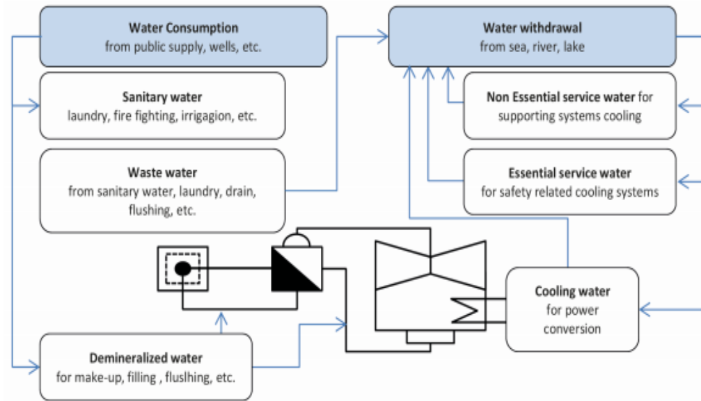
Figure 6-1: Water Streams in an NPP regarding consumption and withdrawal for open loop cooling system
