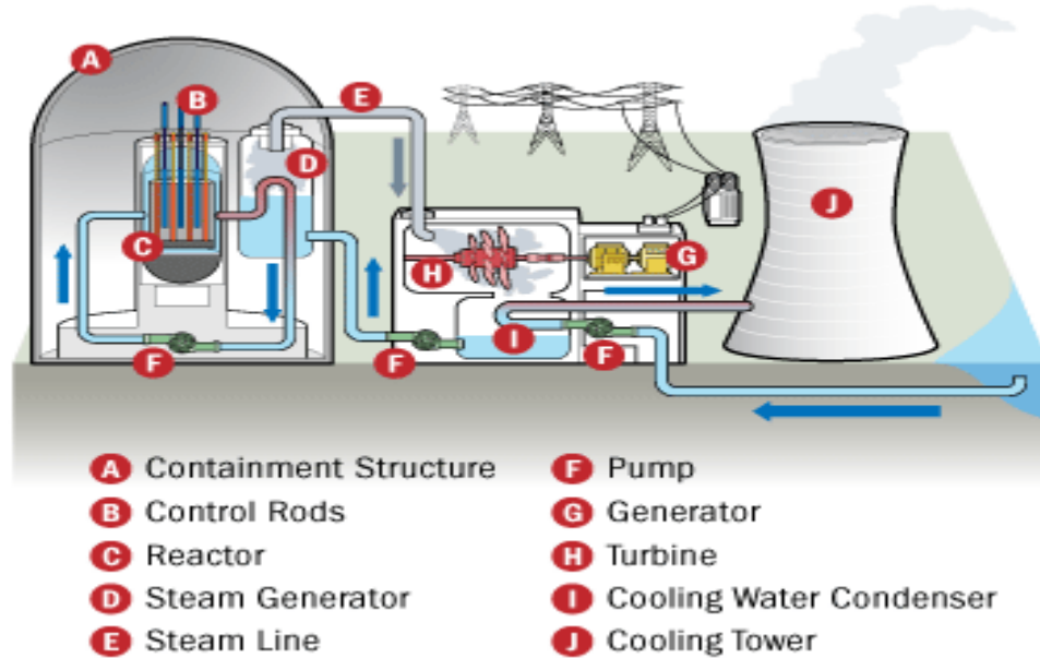
Figure 2-2: Components of a Generation 3 nuclear reactor Source: KIGER, 2019
