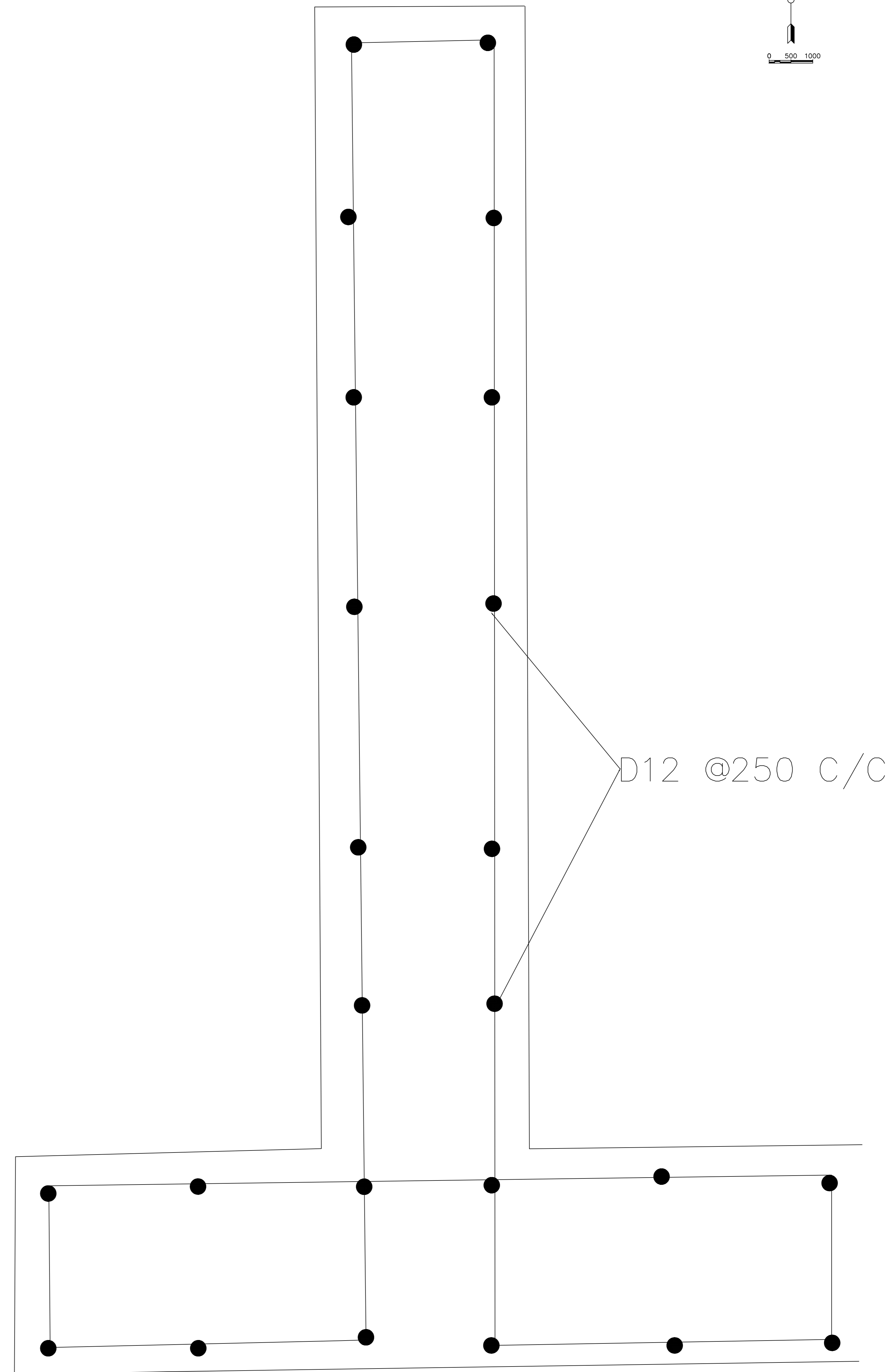
WING WALL REINFORCMENTS
