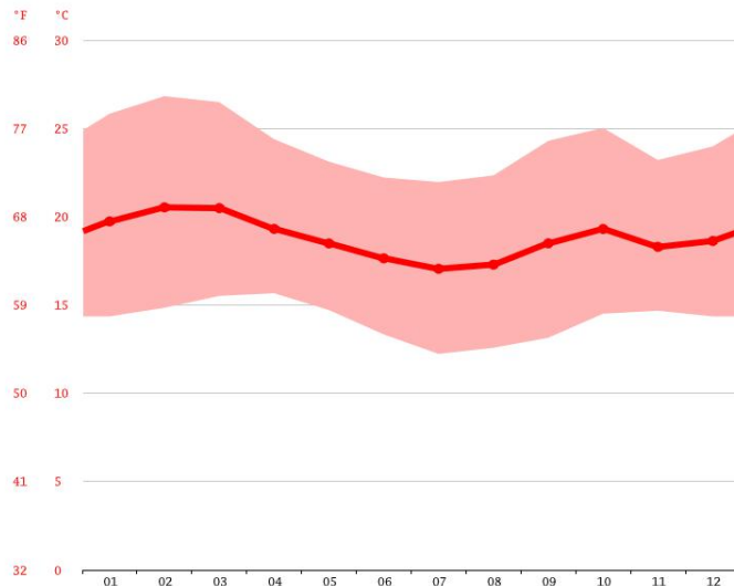
Figure 3: Temperature graph for Nairobi
